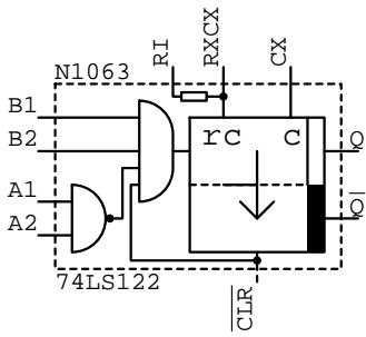
74LS122 N????
