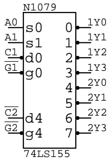
74LS155 N????
