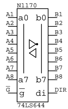
74LS644
