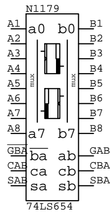
74LS654
