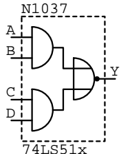
74LS51X N?????
