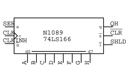
74LS166 N????
