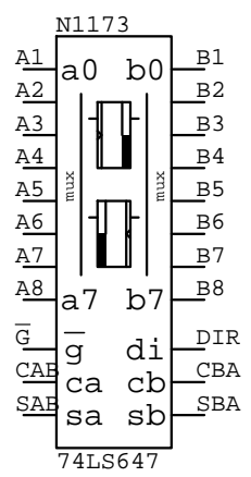
74LS647
