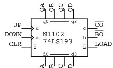
74LS193 N????
