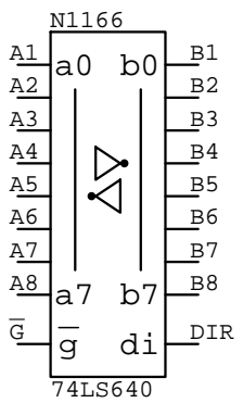
74LS640
