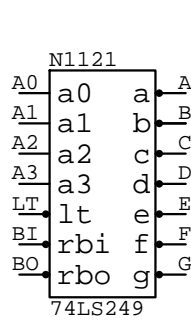
74LS249 N????
