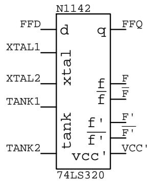
74LS320 N????
