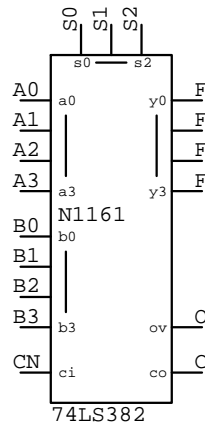
74LS382 N????
