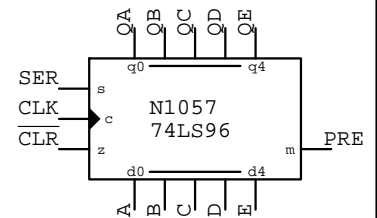
74LS96
