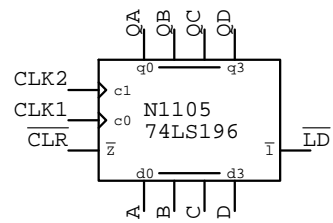
74LS196
