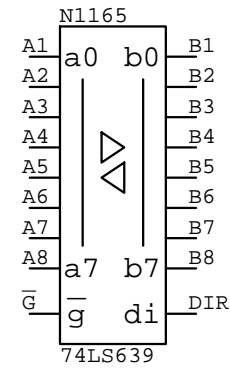
74LS639
