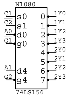
74LS156 N????
