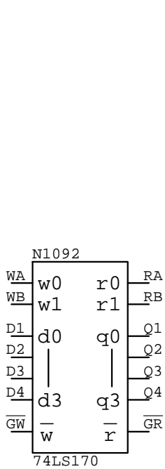
74LS170 N????
