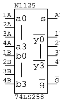
74LS258 N????
