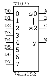
74LS152 N????
