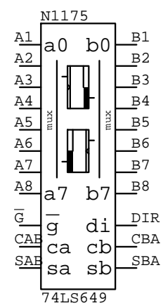
74LS649
