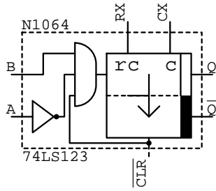
74LS123 N????
