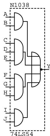
74LS54 N?????
