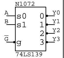
74LS139 N????
