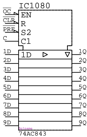
74AC843 IC????
