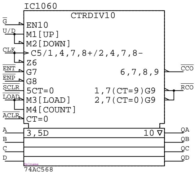
74AC568 IC????
