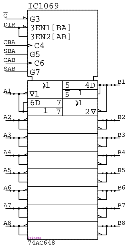
74AC648 IC?????
