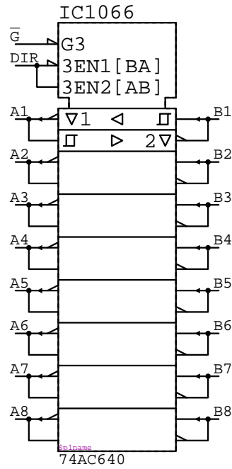
74AC640 IC?????
