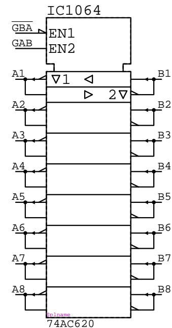
74AC620 IC????
