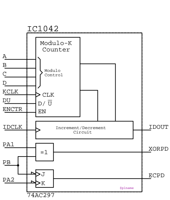
74AC297 IC????
