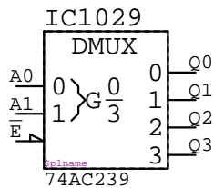
74AC239 IC????
