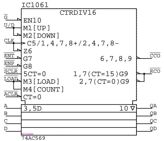
74AC569 IC????
