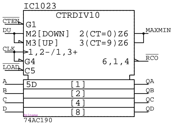
74AC190 IC????
