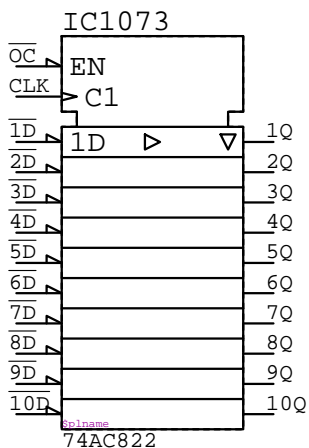
74AC822 IC?????
