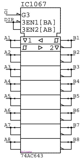
74AC643 IC?????
