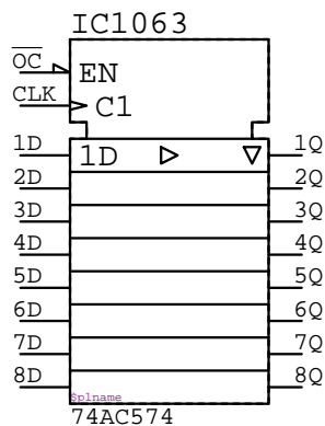
74AC574 IC????
