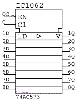
74AC573 IC????
