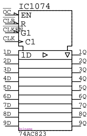
74AC823 IC?????
