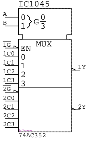
74AC352 IC????
