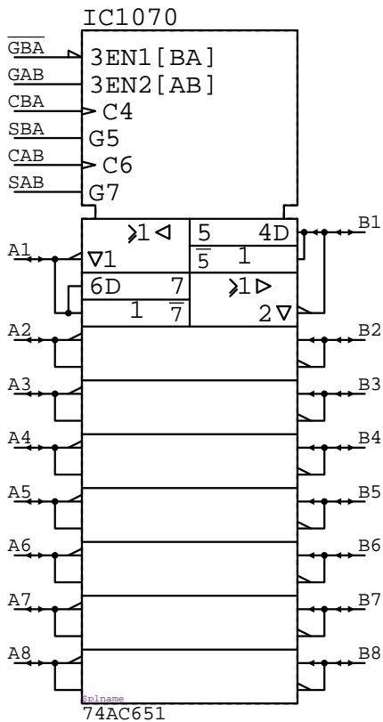
74AC651 IC?????
