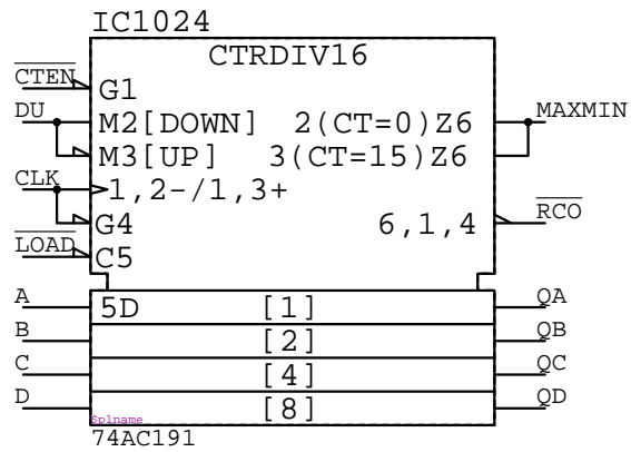
74AC191 IC????
