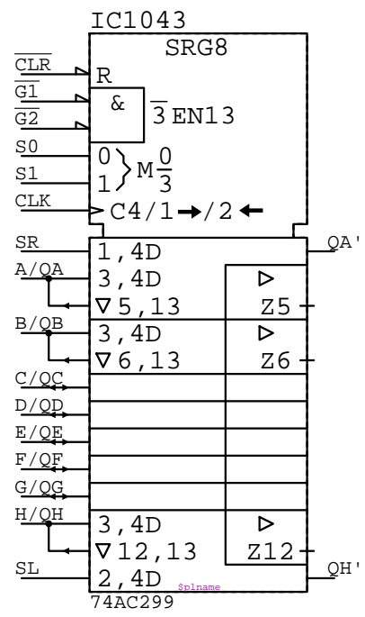
74AC299 IC????
