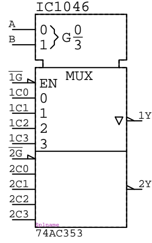
74AC353 IC????
