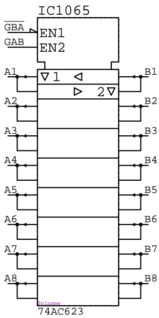
74AC623 IC?????
