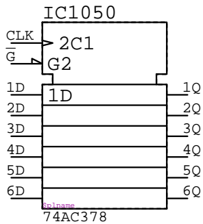
74AC378 IC????
