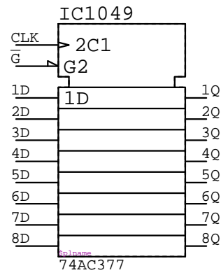
74AC377 IC????
