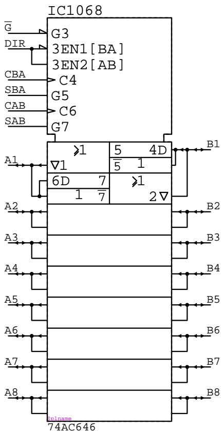
74AC646 IC?????
