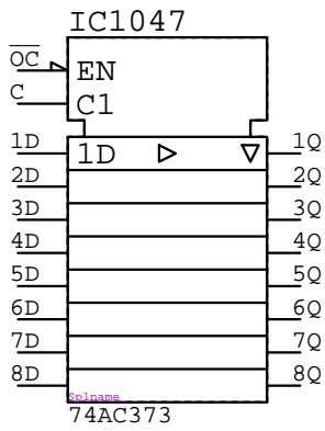
74AC373 IC????
