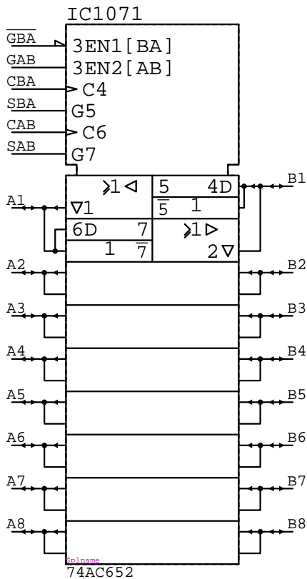
74AC652 IC?????
