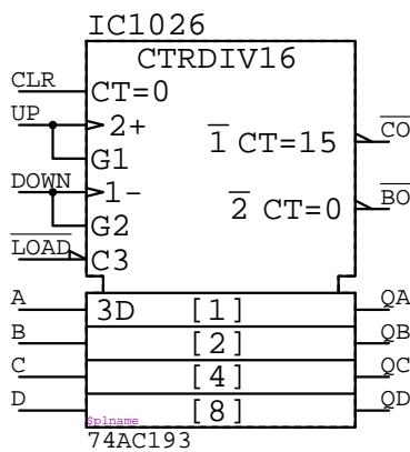
74AC193 IC????
