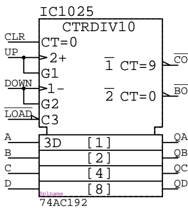
74AC192 IC????
