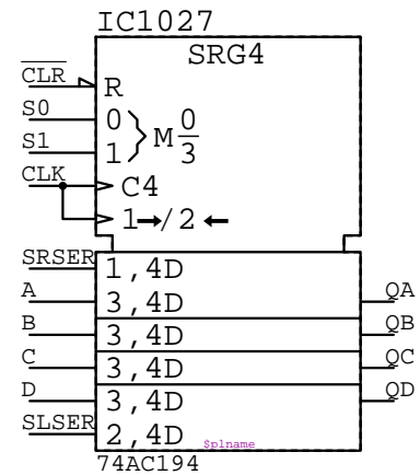
74AC194 IC????
