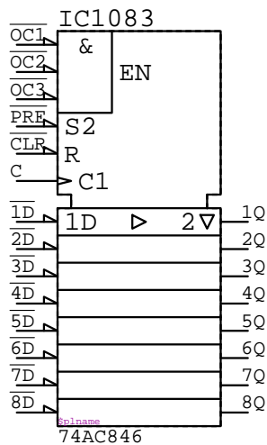
74AC846 IC????
