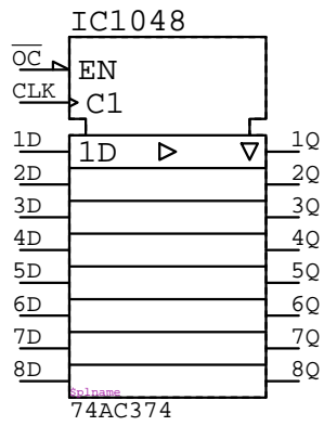
74AC374 IC????
