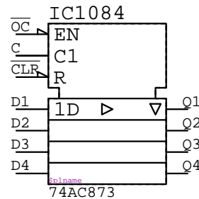
74AC873 IC????
