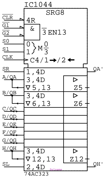
74AC323 IC????
