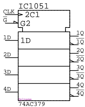
74AC379 IC????
