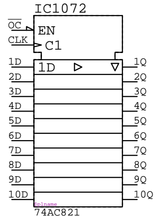
74AC821 IC?????
