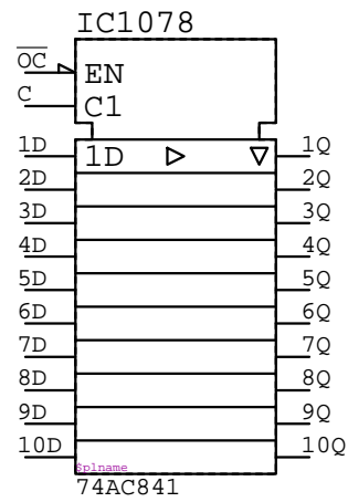
74AC841 IC????
