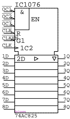
74AC825 IC????
