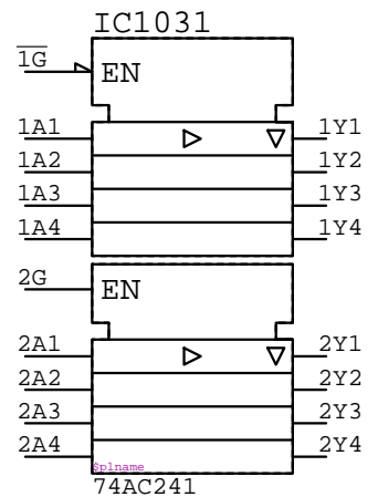
74AC241 IC????
