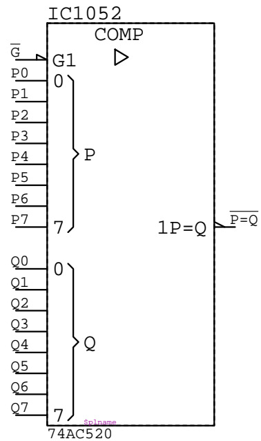
74AC520 IC????
