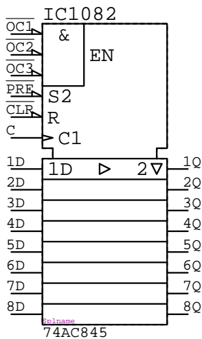
74AC845 IC????
