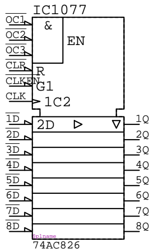
74AC826 IC????
