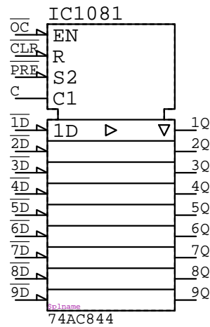
74AC844 IC????
