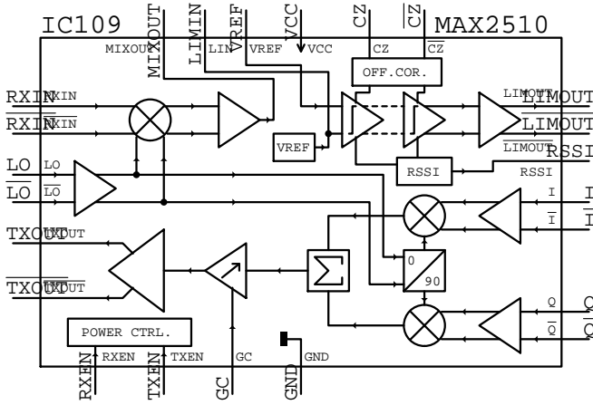
MAX2510 IC???
