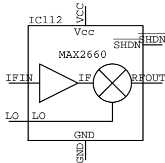
MAX2660 IC???
