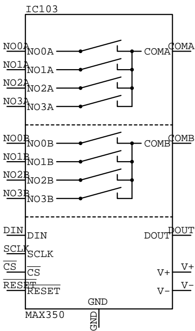
MAX350 IC???
