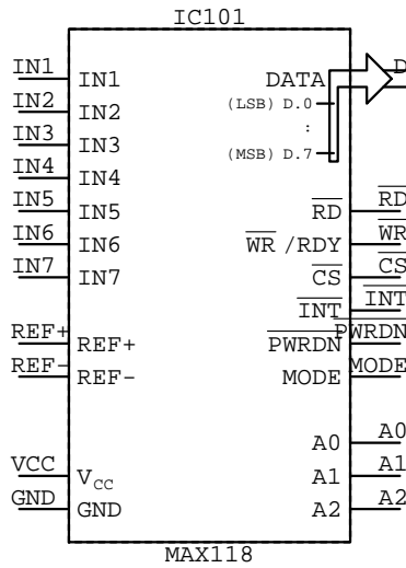
MAX118 IC???
