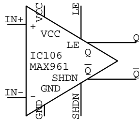
MAX961 IC???
