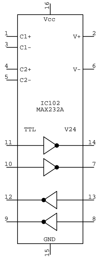
MAX232A IC???
