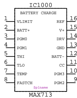
MAX713 IC????
