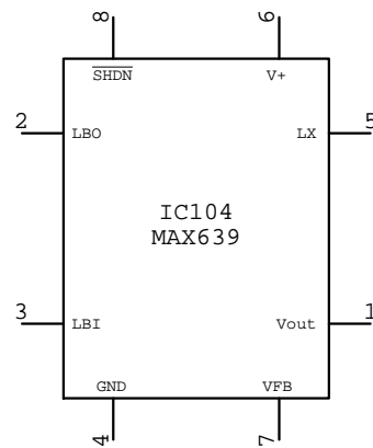
MAX639 IC???
