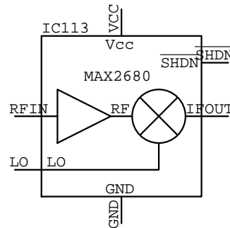
MAX2680 IC???
