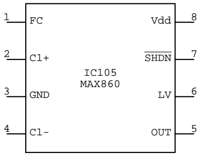
MAX860 IC???
